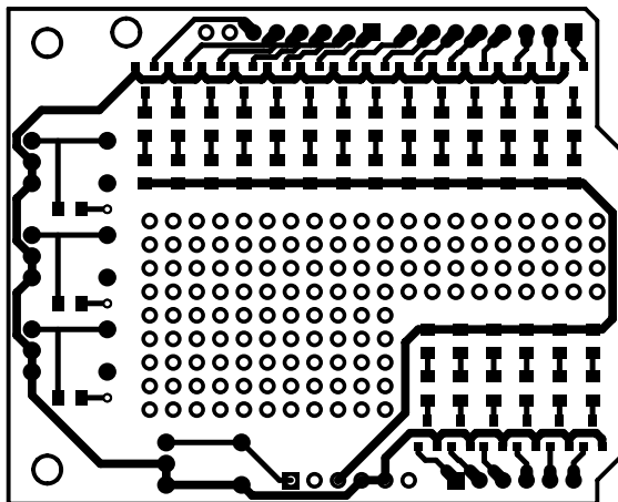
Figure 4. LED Shield PCB Copper Pattern (Top Layer)
