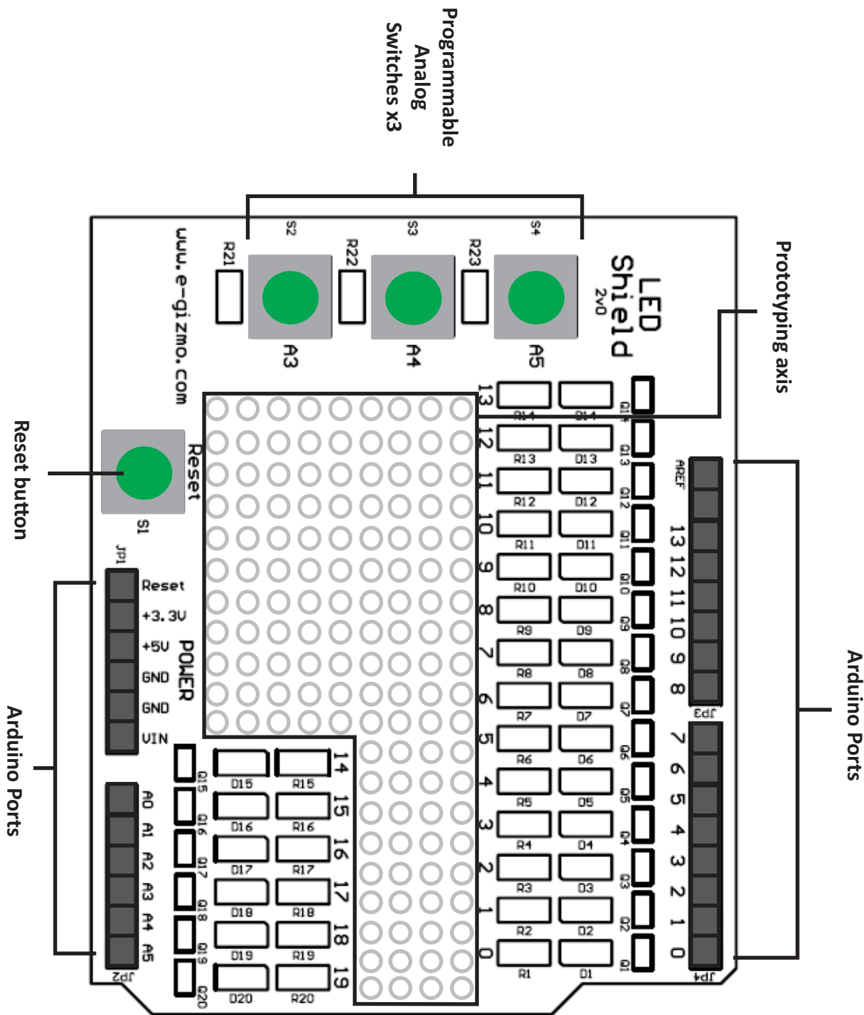
Figure 1. LED Shield 2v0 & its Major Components with Details.
