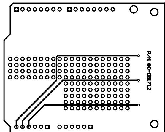
Figure 5. LED Shield PCB Copper Pattern (Bottom Layer)
