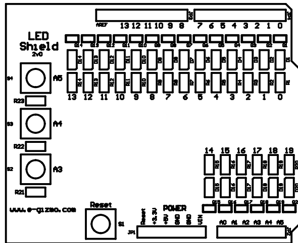
Figure 3. LED Shield 2v0 PCB (Silkscreen layout)
