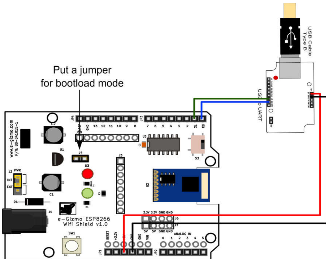
Figure 10 Sample Connections
